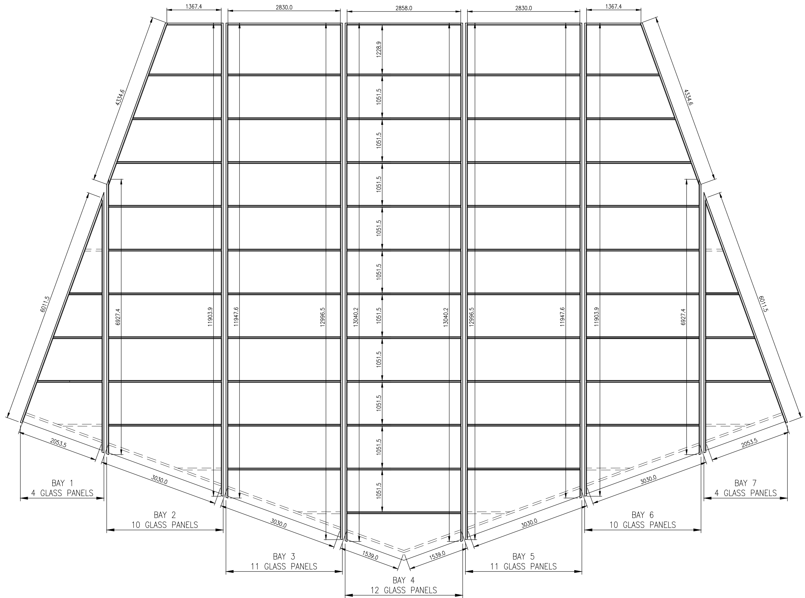
PLAN VIEW OF ATRIUM ROOF GLAZING
